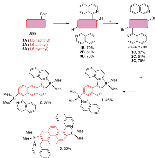
Scheme 2 Synthesis of the dyes 1–3 . (i) 2.6 equiv. 1-chloroisoquinoline, 6 mol% [Pd(PPh 3 ) 4 ], toluene : MeOH (2 : 1), Na 2 CO 3 (aq.), 90 °C. (ii) (1) 2.8 equiv. B 2 pin 2 , 4 mol% [Ir(μ-OMe)(cod)] 2 , 8 mol% 2-pyridinecarboxaldehyde N,N -dibenzylhydrazone, 1,4-dioxane, 90–100 °C. (2) 6.0 equiv. CuBr 2 , i -PrOH : MeOH (2 : 3), water, 90 °C. (iii) (1) 2.4 equiv. n -BuLi, anhydrous THF, –78 °C. (2) 3.0 equiv. Mes 2 BF (Mes: mesityl), –78 °C → rt.
