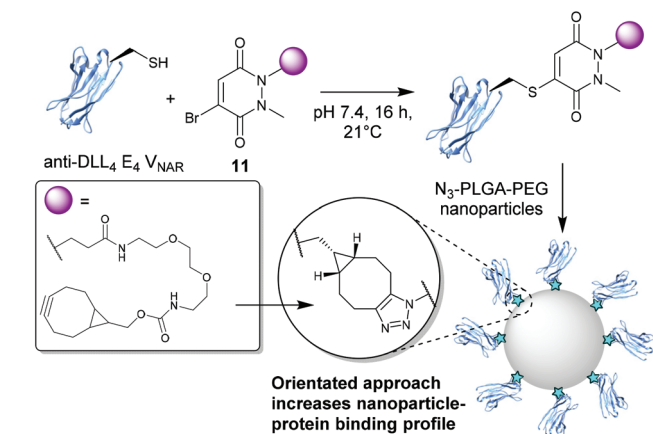
Fig. 5 (a) BrPDs as protecting groups for solid phase peptide synthesis (SPPS). 24 (b) BrPDs facilitate addition of cysteine mutants to the surface of nanoparticles. 37
