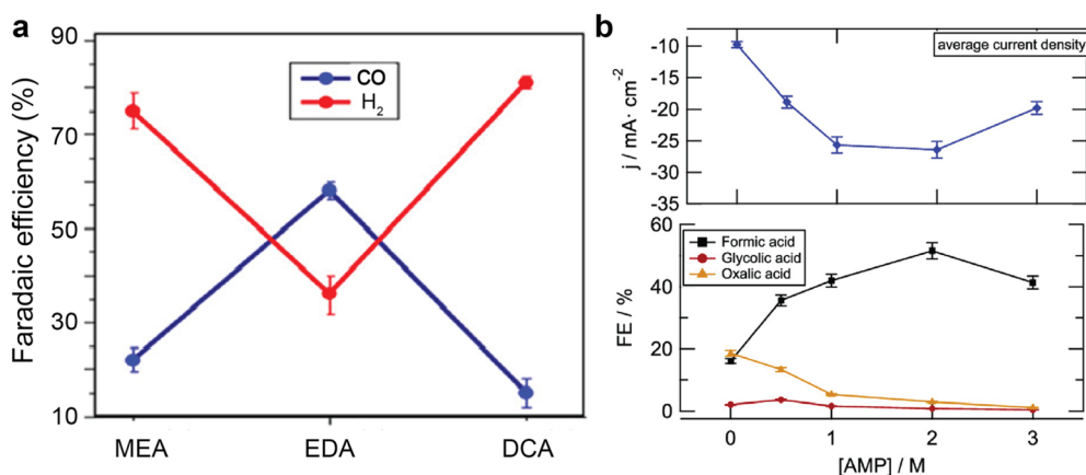
Fig. 10 (a) Faradaic efficiency of CO and H 2 over Cu catalyst in 0.1 M NaClO 4 solution with MEA, ethylenediamine (EDA), and decylamine (DCA) at –0.78 V vs. RHE. Reproduced with permission, 71 copyright 2020, American Chemical Society. (b) The change of current densities and product faradaic efficiency over Pb electrode as a function of 2-amino-2-methyl-1-propanol (AMP) in propylene carbonate solutions at –2.5 V vs. Ag|AgCl at 75 °C. Reproduced with permission, 61 copyright 2021, American Chemical Society.
