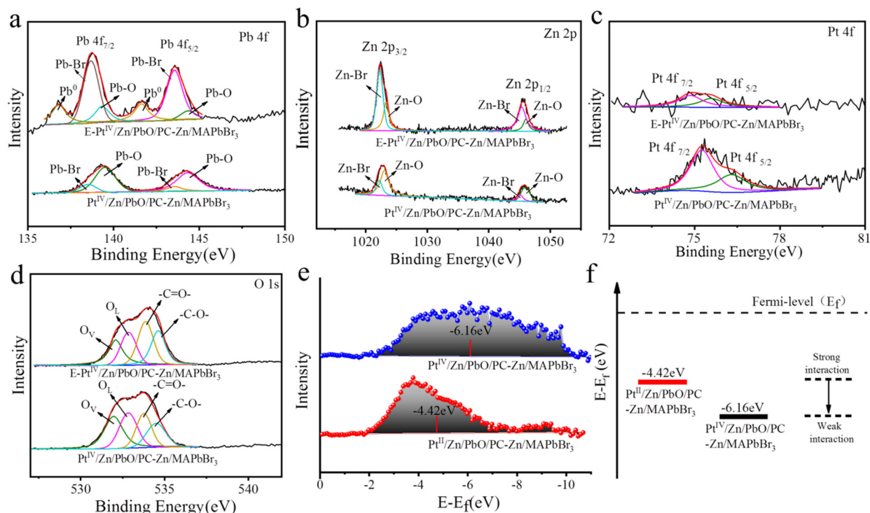
Fig. 3 XPS spectra of Pb 4f (a), Zn 2p (b), Pt 4f (c), and O 1s (d) of non-etched and 20 nm-etched Pt IV /Zn/PbO/PC-Zn/MAPbBr 3 . (e) The d-band center of Pt IV /Zn/PbO/PC-Zn/MAPbBr 3 and Pt II /Zn/PbO/PC-Zn/MAPbBr 3 . (f) Schematic illustrating the shift of the d-band away from the Fermi level to weaken the metal–H interaction. The red and black lines represent their d-band centers.
