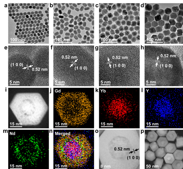
Fig. 1 Transmission electron microscopy (TEM) of (a) \text{NaGdF}_4:\text{Yb},\text{Tm} (CNP), (b) \text{NaGdF}_4:\text{Yb},\text{Tm}@NaYF_4:\text{Yb} (CS1NP), (c) \text{NaGdF}_4:\text{Yb},\text{Tm}@NaYF_4:\text{Yb}@NaGdF}_4:\text{Yb},\text{Nd} (CS2NP) and (d) \text{NaGdF}_4:\text{Yb},\text{Tm}@NaYF_4:\text{Yb}@NaGdF}_4:\text{Yb},\text{Nd}@NaGdF}_4 (DRLNT). (e)–(h) High-resolution TEM (HRTEM) images of core and core–shell nanoparticles in (a)–(d). (i) Scanning transmission electron microscopy (STEM) image of DRLNT. (j)–(n) Energy dispersive X-ray spectroscopy (EDS) elemental mapping of DRLNT showing the distribution of Gd, Y, Yb and Nd elements in the core–multishell structure. (o)–(p) High-angle annular dark field (HAADF)-STEM images of DRLNT.
