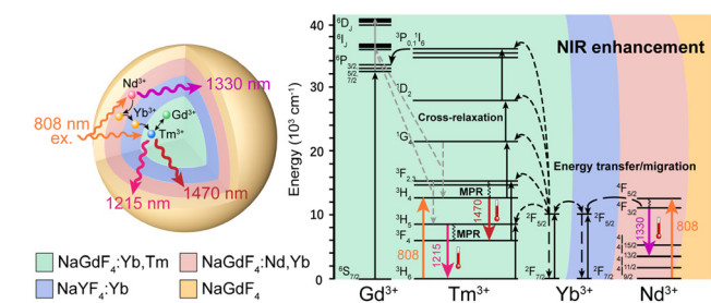
Scheme 1 Schematic of the \text{NaGdF}_4:\text{Yb},\text{Tm}@NaYF_4:\text{Yb}@NaGdF}_4:\text{Yb},\text{Nd}@NaGdF}_4 nanocomposite as a dual ratiometric luminescence nanothermometer (DRLNT). Under the excitation of an 808 nm light source, \text{Nd}^{3+} ions and \text{Tm}^{3+} ions are activated to generate near infrared (NIR) emissions. With the cross-relaxation and phonon-assisted energy transfer processes among lanthanide ions, NIR emissions of DRLNT can be enhanced. The emission at 1215 nm generated from \text{Tm}^{3+} is used as a reference and the emissions at 1470 and 1330 nm from \text{Tm}^{3+} and \text{Nd}^{3+} serve as working wavelengths for temperature sensing.
