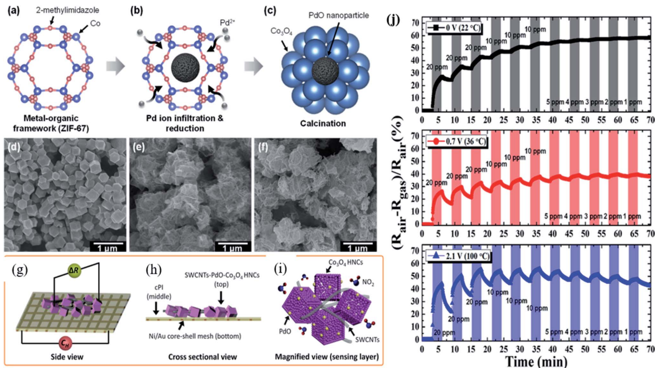
Fig. 13 (a–c) Schematic diagram of PdO loaded Co 3 O 4 Pd/ZIF-67 after annealing at 400 °C, (d–f) SEM image of ZIF-67, PdO-loaded Co 3 O 4 HNCs after calcination, and SWCNT-loaded PdO-Co 3 O 4 HNCs, (g–i) schematic illustration of the fabrication of the SWCNT-loaded PdO-Co 3 O 4 HNC sensor device on a flexible conducting PI film (cPI) with a Ni/Au mesh heater based substrate, and (j) response transients of the SWCNT-loaded PdO-Co 3 O 4 HNC sensor towards NO 2 at different applied voltages (0–2.1 V). Reprinted from ref. 122, copyright@2021, American Chemical Society.
