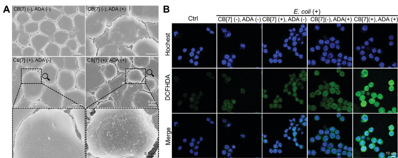
Fig. 2 (A) SEM images of macrophages and E. coli with different formulations (CB[7](−), ADA(−)); (CB[7](+), ADA(−)); (CB[7](−), ADA(+)) and (CB[7](+), ADA(+)) (infected with MOI = 10, 100 min). (B) Intracellular ROS generation of different formulations of the macrophage after infecting E. coli including (CB[7](−), ADA(−)); (CB[7](−), ADA(+)); (CB[7](+), ADA(−)) and (CB[7](+), ADA(+)), respectively, followed by the evaluation of the intracellular ROS by DCFHDA staining and imaging under CLSM.
