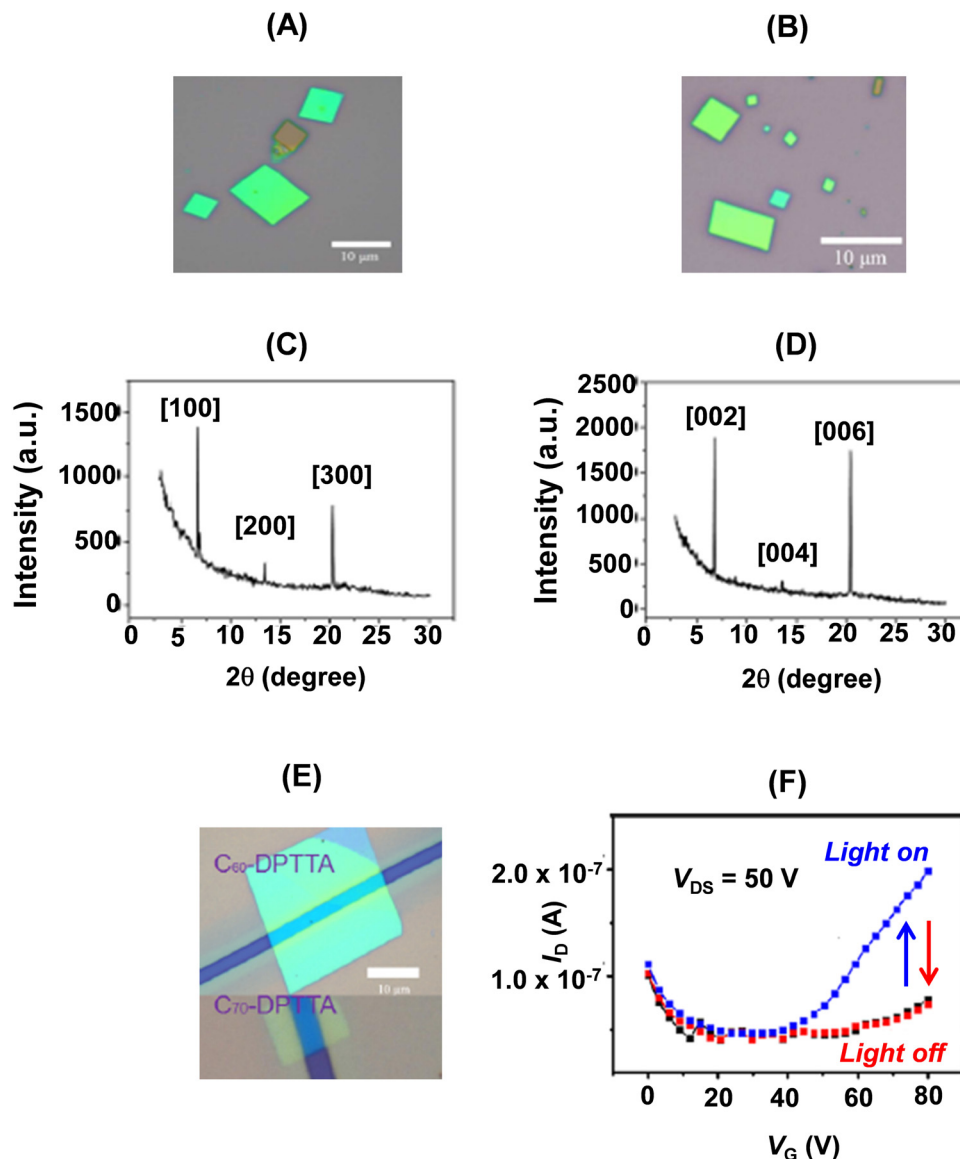
Fig. 15 Optical micrographs of self-assembled 22a - C 60 (A) and 22a - C 70 (B); XRD patterns of 22a - C 60 (C) and 22a - C 70 (D); (E) optical image of the single crystal BGTC devices; (F) photocurrent responses of the 22a - C 70 microcrystal based transistor under light irradiation. Reproduced with permission from ref. 32. Copyright 2013, The American Chemical Society.
