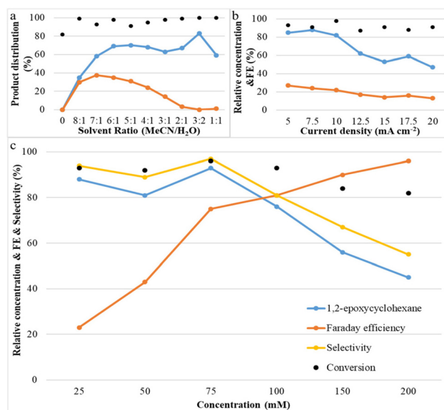
Fig. 3 Reaction conditions: Pt as anode and Pt as cathode, room temperature; (a) different solvent ratios of MeCN and H 2 O: constant current of 10 mA cm -2 , 1a (25 mM), Et 4 NBF 4 (2 eq.), NaBr (1.5 eq.); the ratio of MeCN : H 2 O is varied from 6 : 0 to 1 : 1, 3 h; (b) different current densities: constant current of 5–20 mA cm -2 , 1a (25 mM), Et 4 NBF 4 (2 eq.), NaBr (1.5 eq.), MeCN : H 2 O (3 : 2, 6 ml), 7.46 Faraday mol -1 . (c) different cyclohexene concentrations: 1a from 25–200 mM, constant current of 7.5 mA cm -2 , Et 4 NBF 4 (2 eq.), NaBr (1.5 eq.), MeCN : H 2 O (3 : 2, 6 ml), 4 h.
