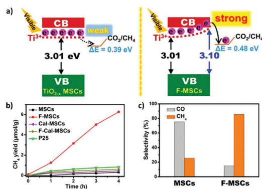
Fig. 14 (a) Schematic illustration of the influence of different Ti 3+ impurity levels between MSCs (mesoporous single crystal) and F-MSCs (Fluorinated MSCs), where \Delta E represents the kinetic overpotential of the reduction process. (b) Time evolution of CH 4 production over various samples under solar light irradiation for 4 h (300 W xenon lamp with an AM 1.5 filter, CO 2 + H 2 O). (c) Selectivity of photocatalytic reduction of CO 2 and H 2 O vapor over MSCs and F-MSCs. Reproduced with permission from ref. 188. Copyright 2018, American Chemical Society.
