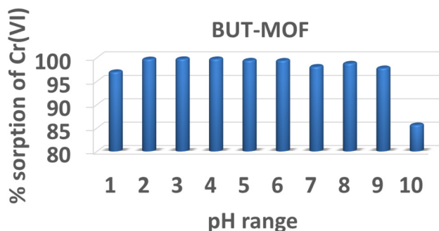
Fig. 4 Percentage (%) sorption of \text{Cr}(\text{vi}) ( 0.1 \text{ mM} ) by BUT-MOF in the \text{pH} range of 1–10.
