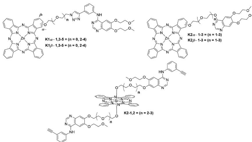
Fig. 11 Phthalocyanines that employ a kinase inhibitor as a targeting vector. Where relevant, the position of attachment of the linker ( \alpha - or \beta -position of the Pc) is indicated in the name; however, each is a single isomer.
