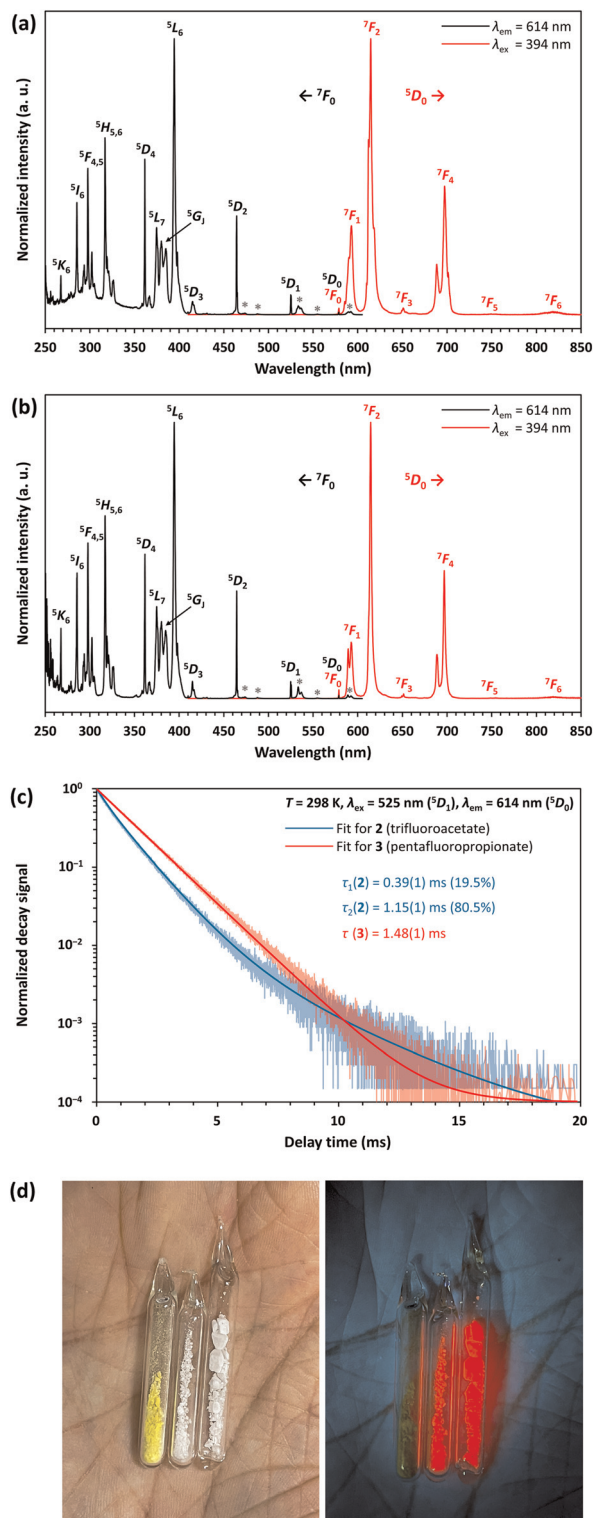
Fig. 9 Excitation (black) and emission (red) spectra of the compounds 2 (a) and 3 (b); excitation lines marked with an asterisk indicate transitions from the thermally populated {}^7F_J ( J = 1, 2 ) levels to the correspondingly labelled levels in the excitation spectrum; (c) luminescence decay of the level {}^5D_0 and fits for 2 and 3 at \lambda_{em} = 614 nm and 298 K; (d) compounds 1 , 2 and 3 in daylight (left) and under a UV lamp with an emission maximum of 265 nm (right). The samples were placed in closed tubes after drying in vacuum.
