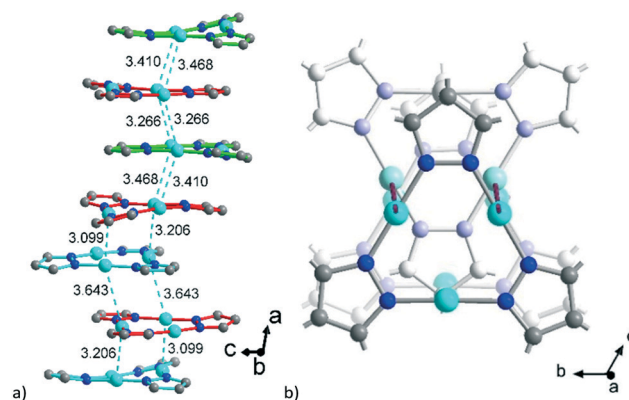
Fig. 4 a) Stacking of the \{Cu_3(pz)_3\} moieties in 1 with Cu^I \cdots Cu^I contacts (in cyan, in Å) between the polycatenated stacks which are differentiated by the same green, red and cyan color as in Fig. 3; the methyl groups are not shown for clarity. b) Alternation of the axial rotation of the \{Cu_3(pz)_3\} moieties.
