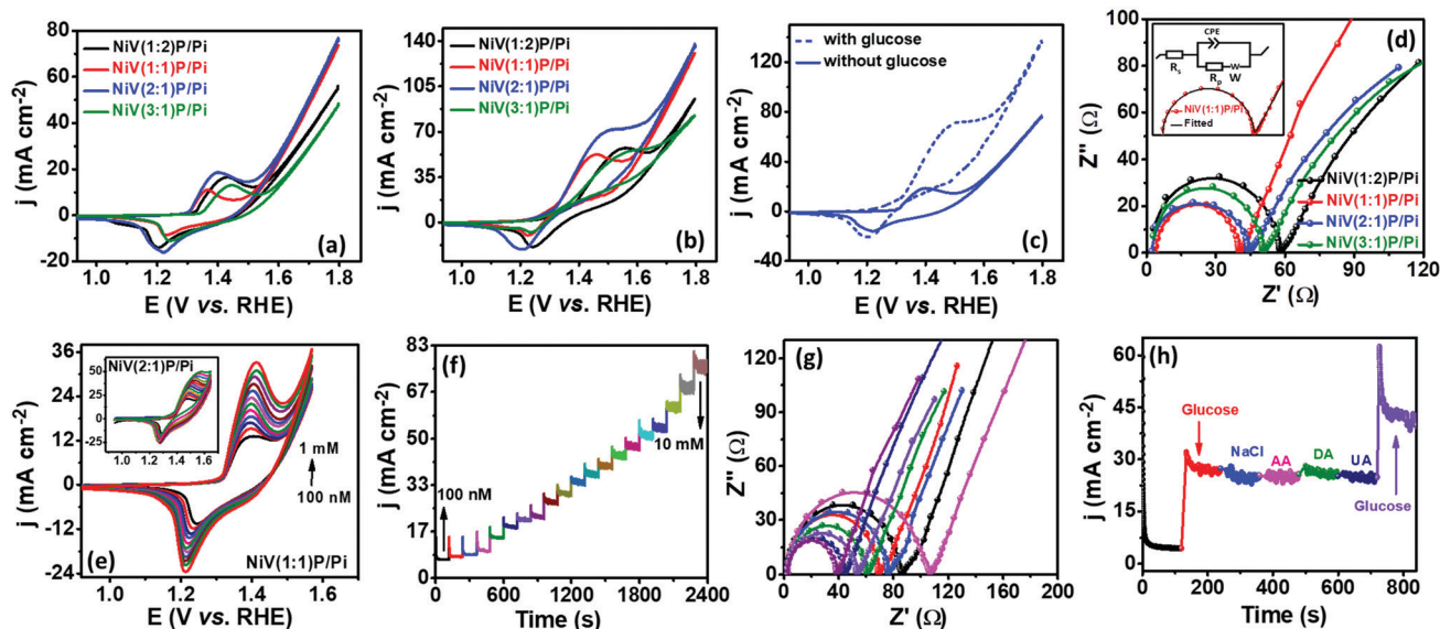
Fig. 2 CV of various NiV(P)/Pi (a) without and (b) with 10 mM of glucose, and (c) comparison of NiV(2:1)/Pi in 0.1 M NaOH electrolyte at a scan rate of 5 \text{ mV s}^{-1} , (d) corresponding EIS studies (inset: fitted equivalent circuit of NiV(1:1)/Pi); (e) CV (inset: CV of NiV(2:1)/Pi), (f) chronoamperometric, and (g) EIS response of NiV(1:1)/Pi on Ni foam in 0.1 M NaOH electrolyte at various conc. of glucose, EIS at frequency ranging from 20 mHz to 3 MHz, (h) chronoamperometric response curve of NiV(1:1)/Pi after the successive addition of 1 mM glucose, 1 mM NaCl, 1 mM AA, 1 mM DA, 1 mM UA and 1 mM glucose in 0.1 M NaOH solution, CE: Pt wire, RE: double junction Ag/AgCl/3 M KCl.
