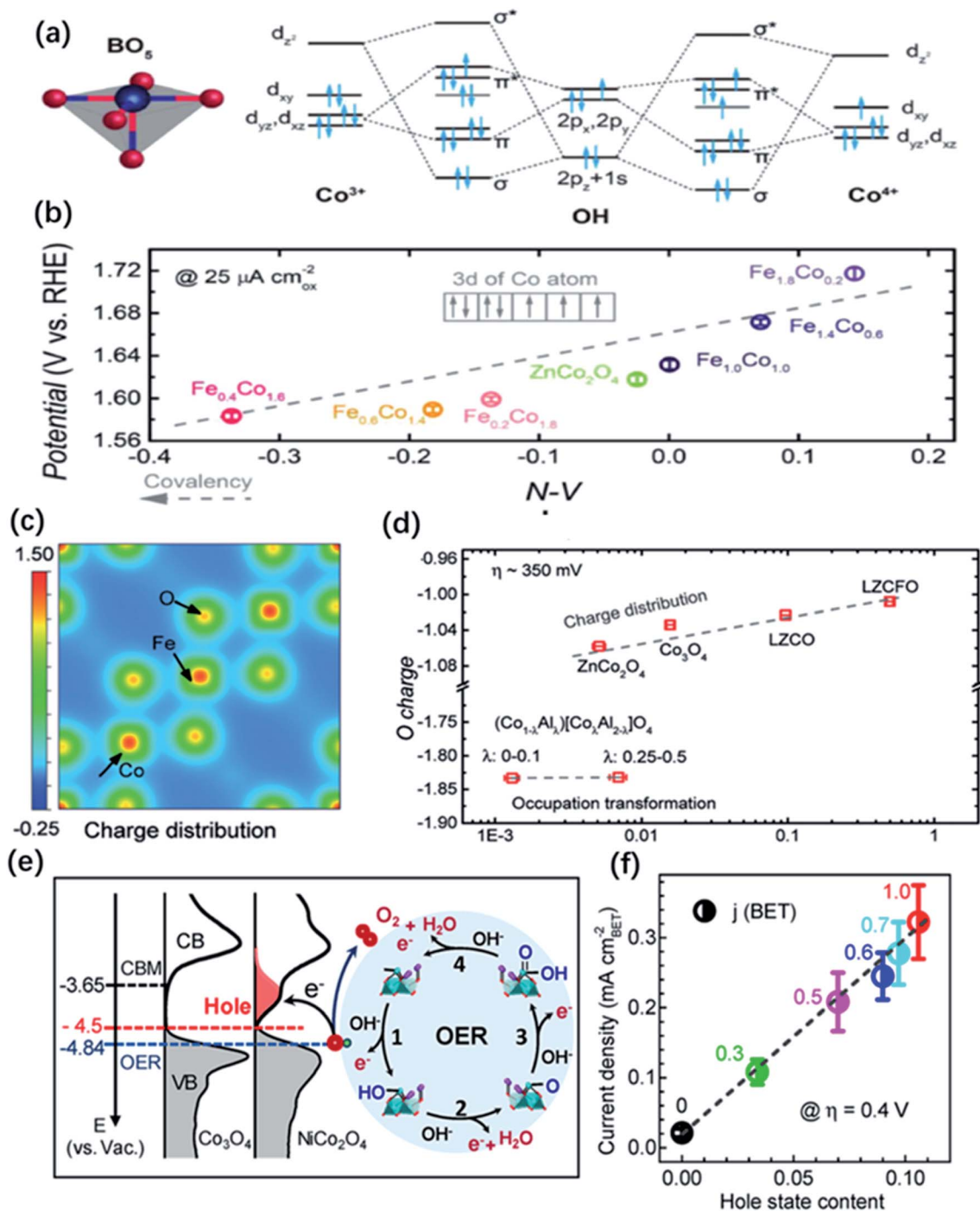
Fig. 11 (a) Molecular orbitals diagrams for the Co–OH (Co 3+ , Co 4+ ) bonding at the surface of spinel oxides. (b) The OER activity, evaluated by the potentials at a current density of 25 \mu\text{A cm}^{-2} , as a function of the N–V parameter. Reproduced with permission. 129 Copyright 2018, Wiley-VCH. (c) Illustration of charge density on [001] direction of LZCFO. (d) OER activity (specific current at an overpotential of \sim 350 mV) as a function of computed oxygen charges. Reproduced with permission. 177 Copyright 2019, Wiley-VCH. (e) Left panel: the measured occupied and unoccupied density of states (DOS) near the E_F for Co 3 O 4 and NiCo 2 O 4 ; the energy level is relative to vacuum level (vs. Vac.). Right panel: schematics of the four-step reaction pathway of OER. (f) Correlation of specific OER activity (current density at \eta = 0.4 V) with the amount of hole state extracted from O K edge XAS spectra. Reproduced with permission. 68 Copyright 2019, American Chemical Society.
