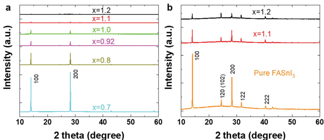
Fig. 1 XRD patterns of \text{PEA}_{0.08}\text{FA}_x\text{SnI}_3 films with (a) x ranging from 0.70 M to 1.20 M and (b) the 1.10 M and 1.20 M patterns compared to the one of pure \text{FASnI}_3 .
