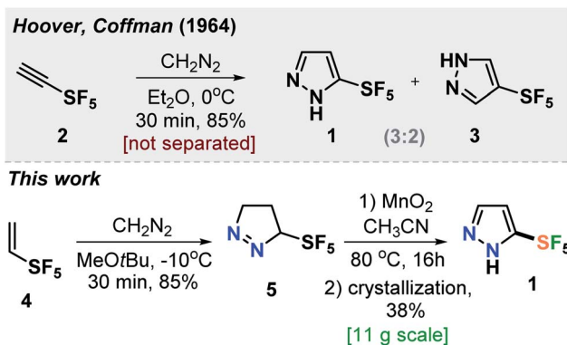
Scheme 1 Synthesis of SF 5 -pyrazole 1 .
