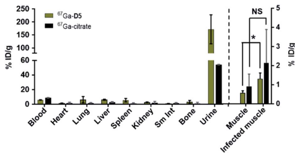
Fig. 6 Comparative biodistribution of ^{67}\text{Ga} Galbifloxacin and ^{67}\text{Ga} -citrate in naive mice ( n = 3 ) shows predominantly renal clearance. (Right to the dotted line) Comparative biodistribution of ^{67}\text{Ga} Galbifloxacin and ^{67}\text{Ga} -citrate in S. aureus infected mice ( n = 3 ). ^{67}\text{Ga} Galbifloxacin shows a significant higher uptake ( P \leq 0.05 ) in the infected muscle as compared to the control muscle ( n = 3 ).
