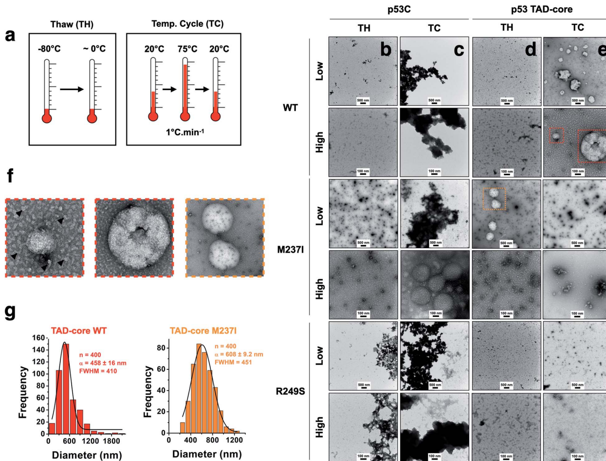
Fig. 4 Influence of intrinsically disordered regions of p53 on the aggregation process. (a) Scheme showing two tested temperature schemes: Thawing (TW) and increase and decrease in temperature (TC). (b–e) Transmission electron micrographs showing the behavior of the wt, M237I and R249S proteins within the context of p53C and p53 TAD-core with respect to solid-like phase transition events at 4 °C (scale bars, 100 and 500 nm). Low and high labels refer to low (scale bar = 500 nm) and high (scale bar = 100 nm) magnification images. (f) Enlarged transmission electron micrographs showing small oligomer-like species (arrowheads). (g) Histogram (bar plots) showing the diameter distribution of droplets of wt and M237I within the context of the p53 TAD-core protein. The data were fitted to a Gaussian distribution (black lines) and show the mean ( \alpha ) \pm s.e.m. of n = 400 measured droplets. FWHM corresponds to full width at half maximum.
