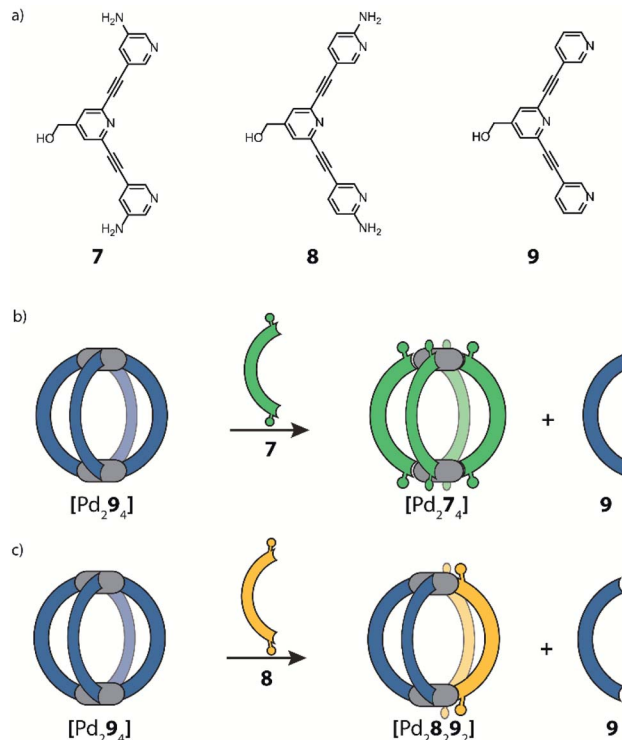
Fig. 6 (a) Banana-shaped ligands bearing amino substituents at the pyridyl donor groups; (b) addition of ligand 7 to [Pd_2L_9]_2 leads to complete displacement of 9 ; (c) formation of heteroleptic cage cis-[Pd_2L_8L_9]_2 can be achieved by partial ligand displacement under kinetic control.
