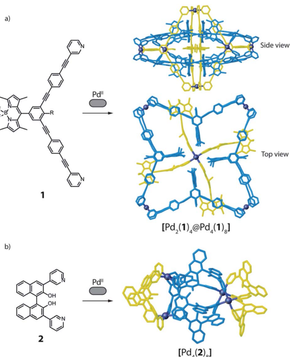
Fig. 3 (a) Ligand 1 self-assembles with Pd II cations to give a cage-in-ring architecture, where 1 occupies two different positions; (b) distorted tetrahedron obtained from a mixture of Pd II and 2, where the ligand positions are not equivalent.
