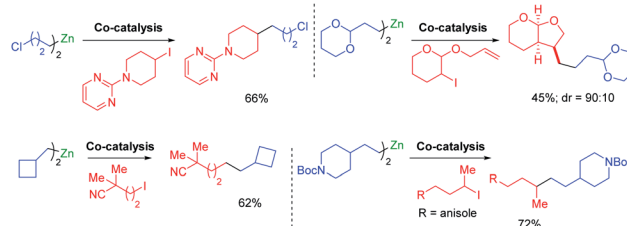
Scheme 10 Cobalt-catalyzed alkyl–alkyl cross-couplings using organozinc reagents.
