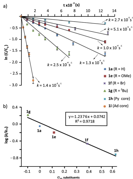
Fig. 3 Cyclization of rotaxanes 1a and 1e – i in the presence of CsOH (1 equiv.) at 25 °C in DMF: (a) Plots of \ln(c/c_0) versus time for the determination of the rate constants; (b) Hammett plot of \log(k/k_{1a}) against the substrate electronics ( \sigma_m ). The rate constant values are the average of two independent measurements.
