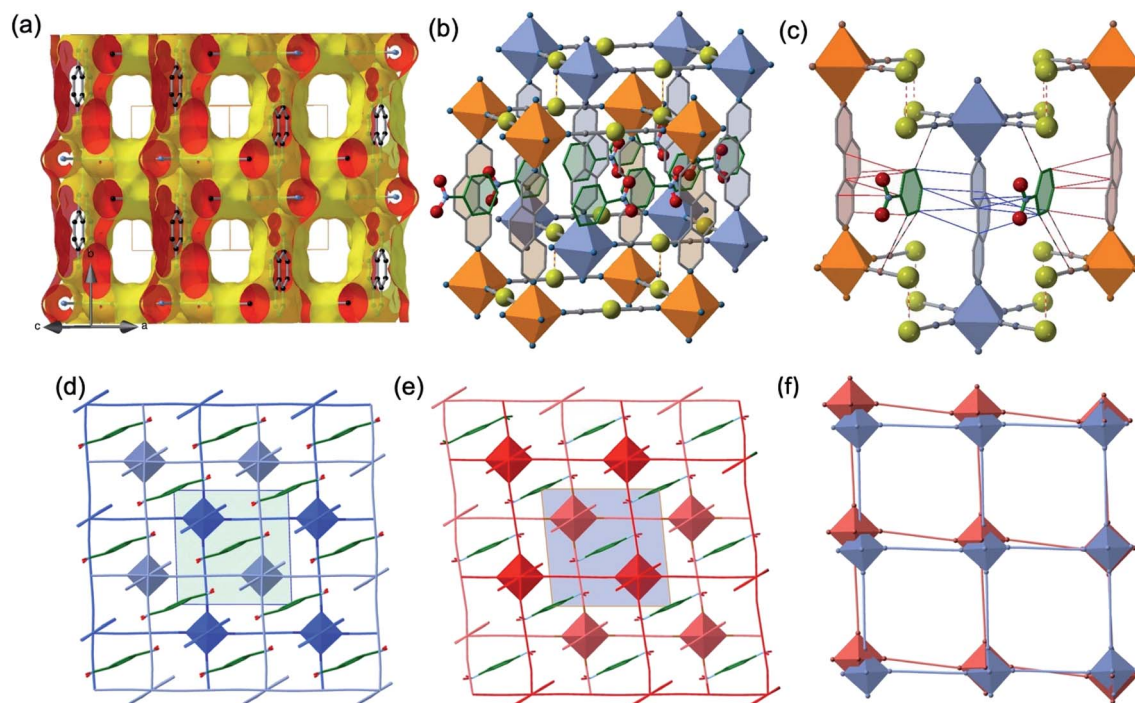
Fig. 4 (Top) View of a fragment of the interpenetrated pcu frameworks illustrating: (a) the solvent-excluded surface showing void channels running along a + c direction; (b) the 1\text{-PhNO}_2 molecules located in the channels (the shown \text{PhNO}_2 molecule represents the average of two slightly disordered positions); and (c) \text{C}_{(3,8\text{-phen})}\cdots\text{C}_{(\text{PhNO}_2)} (red, blue thin bonds) and \text{C}_{(\text{Au}(\text{CN})_2)}\cdots\text{C}_{(\text{PhNO}_2)} (black-red thin bonds) intermolecular interactions shorter than the sum of van der Waals radii at 228 K. Red-white thin bonds correspond to the Au \cdots Au interactions between the two interpenetrated frameworks. (Bottom) View down to [010] direction of the interpenetrated frameworks marked in light- and dark-blue LS state (d), light- and dark-red (HS state) (e) including the \text{PhNO}_2 molecule located in the channels (the inner green/blue squares correspond to the unit cell); (f) superposition of one of the two frameworks illustrating the distortion of the structure when moving from the LS state (blue) to the HS state (orange).
