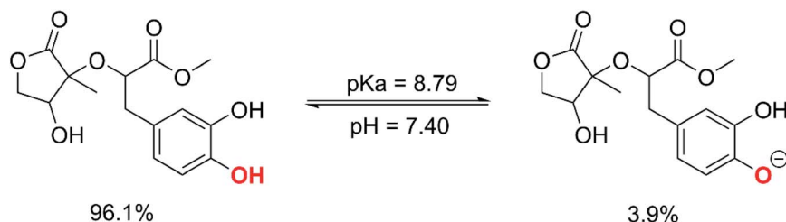
Fig. 4 The deprotonation of MO at pH = 7.4.
