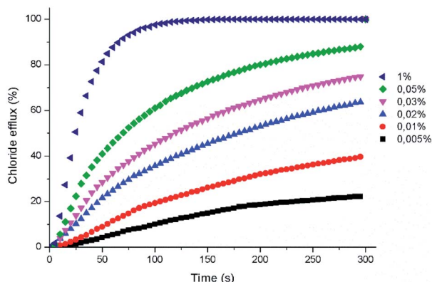
Fig. 3 Chloride efflux promoted by 4T at different concentrations (1–0.005% carrier to POPC molar ratio, 5–0.025 \mu\text{M} ) in unilamellar POPC vesicles. Vesicles loaded with 489 mM NaCl were buffered at pH 7.2 with 5 mM phosphate and dispersed in 489 mM \text{NaNO}_3 buffered at pH 7.2. Each trace represents the average of at least three trials.
