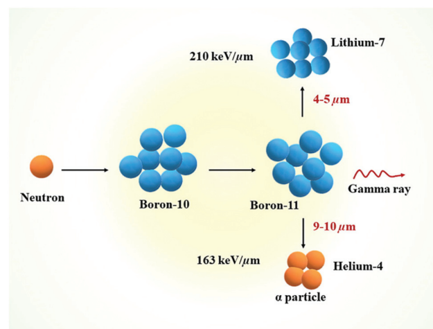
Fig. 1 Schematic representation of the nuclear reaction that happens during the BNCT process. Reproduced from ref. 2 with permission from Elsevier, copyright 2020.
