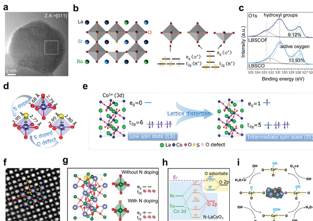
Fig. 8 (a) HRTEM image of LBSCOF. (b) Schematic representation of the perovskite oxide structure and featured [\text{CoO}_6]_{\delta} polyhedron. (c) XPS spectra of O 1s for LBSCOF and LBSCO. Reproduced with permission from ref. 60. Copyright 2018, Elsevier Inc. (d) Schematic representation for optimized atomic structures. (e) Schematic representation of the evolution of the IS state and the transition of electrons from t_{2g} to e_g orbital. Reproduced with permission from ref. 109. Copyright 2020, American Chemical Society. (f) ABF-STEM image of N-LCO. (g) Spin density distribution and electronic configuration of LCO and N-LCO. (h) Schematic representation of orbital bonding. (i) Illustration diagram of the four-step process of the OER. Reproduced with permission from ref. 62. Copyright 2021, American Chemical Society.
