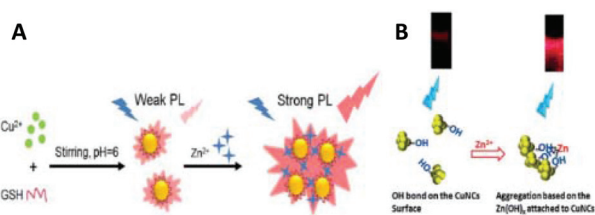
Fig. 21 (A) Schematic illustration of the preparation of GSH-capped CuNCs and the aggregation-induced PL enhancement of CuNCs in the presence of Zn 2+ . Reprinted with permission from ref. 225. Copyright 2017 Elsevier. (B) Scheme for the mechanism of the aggregation-induced fluorescence enhancement for CuNCs in the presence of Zn 2+ . Republished with permission from ref. 110. Copyright 2016 Royal Society of Chemistry.
