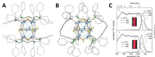
Fig. 7 Molecular structure of (A) [\text{Cu}_{12}\text{S}_6(\text{dpdp})_4] and (B) [\text{Cu}_{12}\text{Se}_6(\text{dpdp})_4] clusters. Colour codes of the elements: Cu: blue, S: yellow, P: green and C: grey. H atoms are omitted for clarity. (C) Room temperature photoluminescence excitation (PLE) and emission (PL) spectra of a suspension of freshly prepared microcrystals of [\text{Cu}_{12}\text{S}_6(\text{dpdp})_4] (down) and [\text{Cu}_{12}\text{Se}_6(\text{dpdp})_4] (up) in toluene, measured in the integrating sphere. The inset shows the colours of the suspensions of microcrystal under white LED light. Republished with permission from ref. 164. Copyright 2014 Royal Society of Chemistry.
