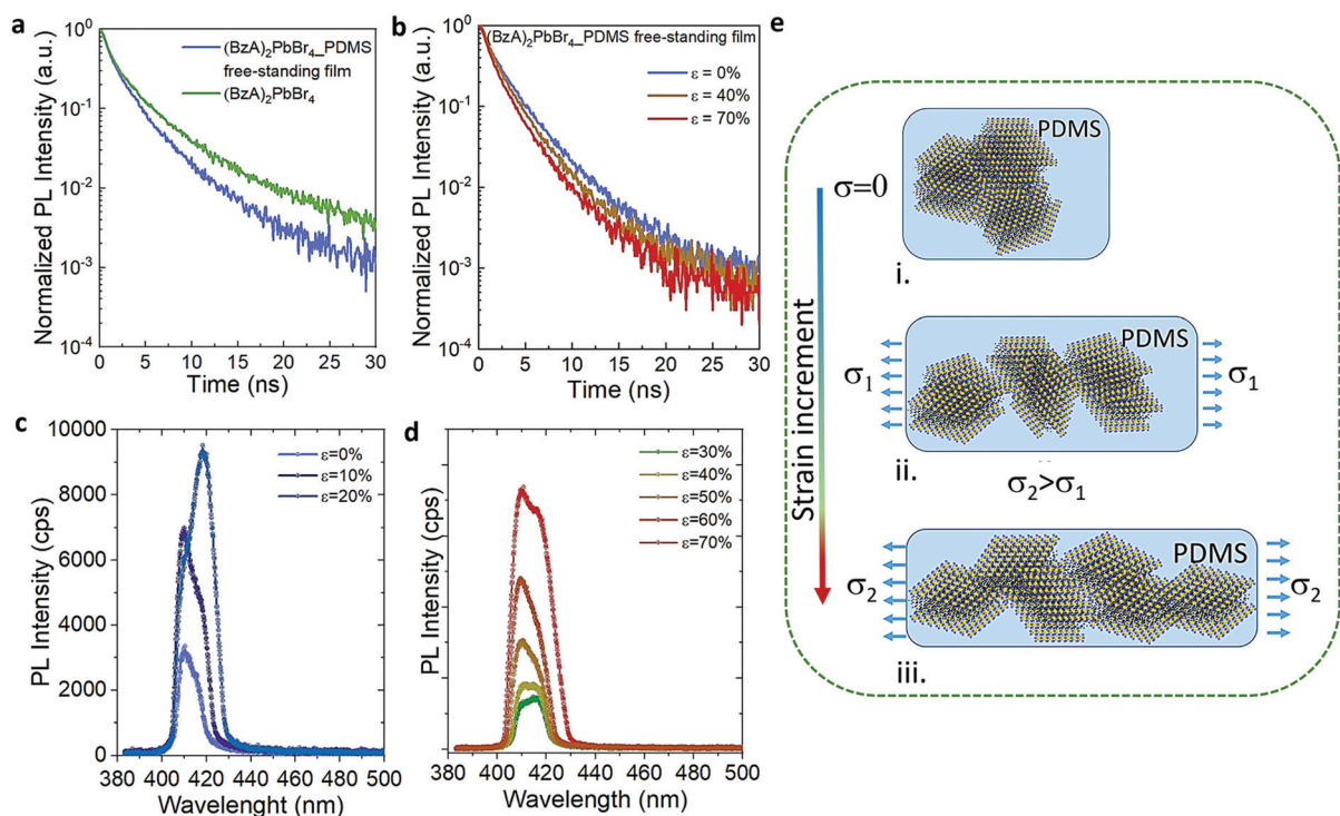
Fig. 3 (a and b) PL decay profiles collected from a deposit of the (BzA) 2 PbBr 4 platelets (green), and the (BzA) 2 PbBr 4 -PDMS free-standing film (blue) without stretching in (a) and under stretching up to 70% in (b). (c and d) Emission spectra collected from the films by applying step-by-step stretching. (e) Cartoon explaining the orientation switching of the platelets in the polymer film under continuous tensile strain: (i) without stretching, the platelets are stacked one on top of the other and randomly oriented in the film; (ii) under an initial stress ( \sigma_1 ), the ensemble of platelets start to separate from each other and adopt a preferential orientation parallel to the applied stress; (iii) by increasing the stress ( \sigma_2 ), preferentially oriented ensembles become more separated and a sliding of platelets within the ensembles takes place, providing thinner structures in the film, from which an enhanced PL intensity is observed.
