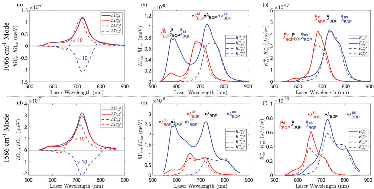
Fig. 4 Dependence of (a and d) the vibrational frequency shift parameters \Omega_{\text{vp}}^{\pm, c} , \Omega_{\text{vp}}^{\pm, s} , (b and e) the vibrational pumping \Gamma_{\text{vp}}^{+, c} , \Gamma_{\text{vp}}^{+, s} and damping \Gamma_{\text{vp}}^{-, c} , \Gamma_{\text{vp}}^{-, s} rates, and (c and f) the propagation factors K_{\text{vp}}^{\pm, c} , K_{\text{vp}}^{\pm, s} , on the wavelength of the illuminating laser of intensity I_{\text{las}} = 1 \mu\text{W} \mu\text{m}^{-2} and Raman-active vibrational mode of wave-number (a–c) 1066 \text{cm}^{-1} and (d–f) 1586 \text{cm}^{-1} . The solid lines are computed with the continuum-field model (labeled by “c”) while the dashed lines are calculated with the single-mode model (labeled by “s”). In (b and c), the dots from right to left mark the laser wavelengths where the anti-Stokes emission ( \lambda_{\text{BDP}}^{\text{st}} = 780 \text{ nm} ), the excitation ( \lambda_{\text{BDP}} = 720 \text{ nm} ), and the Stokes emission ( \lambda_{\text{BDP}}^{\text{st}} = 669 \text{ nm} ) are maximized due to the BDP mode. The squares mark the same information ( \lambda_{\text{BQP}}^{\text{st}} = 618 \text{ nm} , \lambda_{\text{BQP}} = 580 \text{ nm} , \lambda_{\text{BQP}}^{\text{st}} = 546 \text{ nm} ) for the BQP mode. In (e and f), the dots and squares mark the same information as in (b and c) for the high-energy vibrational mode with values of \lambda_{\text{BDP}}^{\text{st}} = 813 \text{ nm} , \lambda_{\text{BDP}} = 720 \text{ nm} , and \lambda_{\text{BDP}}^{\text{st}} = 646 \text{ nm} for the BDP mode, and \lambda_{\text{BQP}}^{\text{st}} = 639 \text{ nm} , \lambda_{\text{BQP}} = 580 \text{ nm} , and \lambda_{\text{BQP}}^{\text{st}} = 531 \text{ nm} for the BQP mode. The difference between the wavelengths marked in (b and c) and (e and f) are due to the difference in the vibrational energy, which affects the Stokes and anti-Stokes frequencies. The results for the 1269 \text{cm}^{-1} mode are shown in Fig. S4 of the ESI.† Other parameters are specified in the text.
