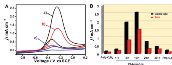
Fig. 8 (A) Cyclic voltammogram of Pt-Au (10 : 1)/g-C 3 N 4 (a) and Pt/g-C 3 N 4 (c) electrodes under visible-light illumination (a) and under dark (b and c), respectively. (B) The histogram of activities of different electrodes with different ratio of Pt and Au for MOR upon visible light and dark environment. This figure has been adapted from ref. 104 with permission from Elsevier, copyright 2020.
