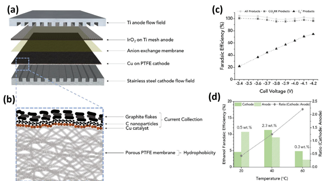
Fig. 14 Exploded view of MEA layers inside the electrolyzer (a) where the hatched line box is the Cu on PTFE cathode with the cross-section structure is displayed in (b); (c) faradaic efficiencies of all products (H 2 and EC CO 2 R) and C 2+ products and (d) amounts and ratios of FE ethanol that are recovered from the cathode and anode streams at each temperature. Reproduced from ref. 139 with permission of Joule.
