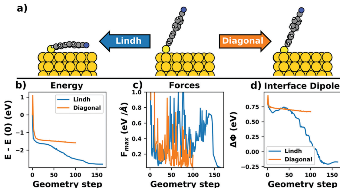
Fig. 20 Geometries of a cyano-biphenylthiol molecule on Au(111), calculated in a 5 \times 2\sqrt{3} unit cell with FHI-aims using the PBE+vdW surf method and a 3 \times 2 \times 1 -centered k -point grid. A three-layer metal slab was used. All atoms of the molecule and the topmost layer of the slab were allowed to relax until the remaining forces on all atoms fell below 0.01 \text{ eV \AA}^{-1} . The calculations can be found on the NOMAD database. [https://dx.doi.org/10.17172/NOMAD/2020.12.07-9]. (a) Shows the starting geometry (center) and the final result after the optimization using a diagonal guess for the Hesse matrix (right) or using a Lindh guess (left). (b) Shows the evolution of the total energy relative to the energy of the starting point, for the two geometry optimizations. (c) Shows the remaining maximum force component F at each iteration step, (d) gives the interface dipole \Delta\phi .
