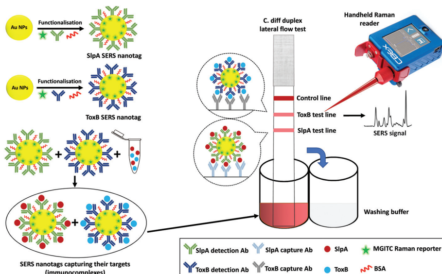
Fig. 1 Schematic representation for the duplex detection of SIpA and ToxB by SERS-based LFA.
