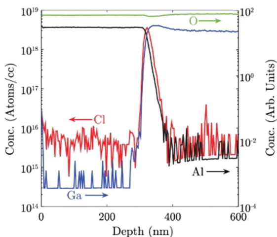
Fig. 3 Cl concentration in atoms per cc and Ga, Al and O concentration in arbitrary units, measured by SIMS for an \alpha\text{-Ga}_2\text{O}_3 sample grown by HVPE at 650 °C. Reproduced from ref. 53.
