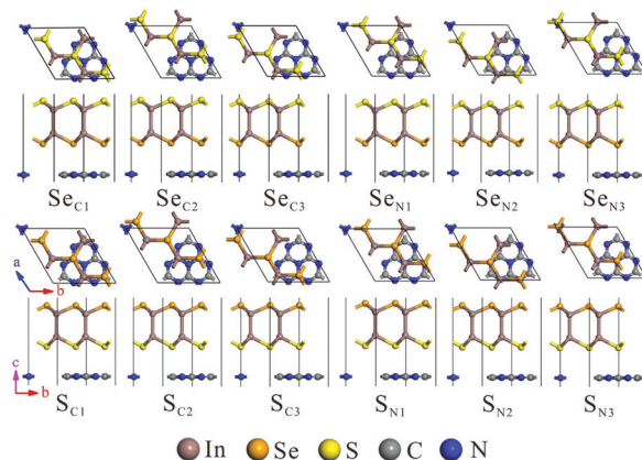
Fig. 1 Top and side views of the \text{In}_2\text{SeS/g-C}_3\text{N}_4 heterostructure at different stacking patterns: \text{Se}_{\text{C}1} , \text{Se}_{\text{C}2} , \text{Se}_{\text{C}3} , \text{Se}_{\text{N}1} , \text{Se}_{\text{N}2} , \text{Se}_{\text{N}3} , \text{S}_{\text{C}1} , \text{S}_{\text{C}2} , \text{S}_{\text{C}3} , \text{S}_{\text{N}1} , \text{S}_{\text{N}2} and \text{S}_{\text{N}3} .
