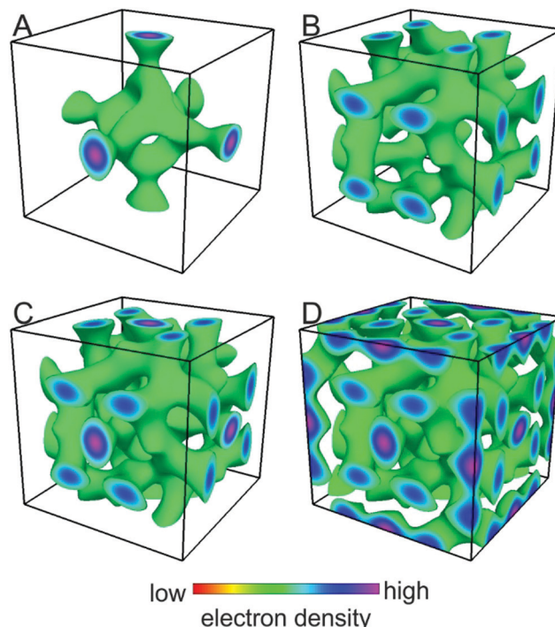
Fig. 6 Reconstructed electron density maps of the triple network cubic phase with space group symmetry I23 . The green isosurfaces enclose the high density (aromatic) regions of the 3D electron density map. (A) Inner network; (B) middle network; (C) inner and middle networks; (D) inner, middle and outer networks.
