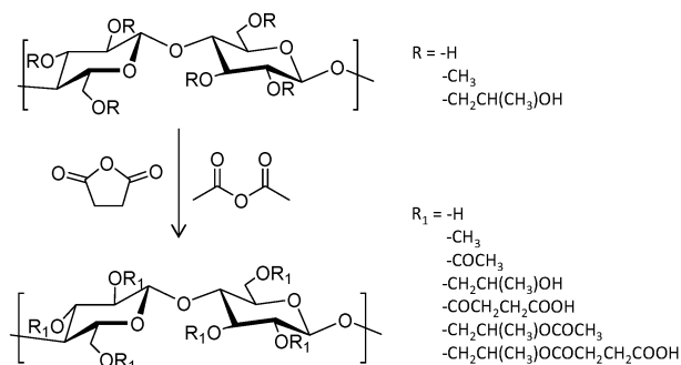
Fig. 6 General reaction scheme to convert HPMC polymers to HPMC-AS through the addition of acetyl and succinyl groups. 105
