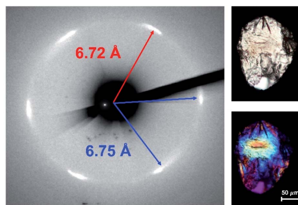
Fig. 3 (Left) Hexagonal six-fold X-ray diffraction pattern obtained for the functionalized nanothread; and (right) 50× images within a stainless-steel gasket, illustrating crystallinity along with (bottom) a polarized light micrograph using a 530 nm waveplate.
