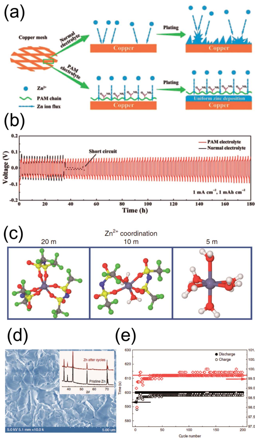
Fig. 3 (a) A schematic illustration of Zn plating on Cu mesh with a normal aqueous electrolyte and that with a PAM additive. (b) Galvanostatic voltage profiles of Zn symmetric cells with (red) and without (black) the PAM additive at 1 mA h cm -2 . (a and b) Reprinted with permission from ref. 34. Copyright 2019, Wiley-VCH. (c) Molecular dynamics simulations of Zn 2+ coordination in different LiTFSI concentrations (20, 10, and 5 M). (d) SEM image of plated Zn in a high concentration electrolyte (20 M LiTFSI & 1 M ZnTFSI); inset: ex situ XRD profile of pristine (black) and cycled Zn (red). (e) Plating test results on Cu in a high concentration electrolyte. (c–e) Reprinted with permission from ref. 43. Copyright 2018, Springer Nature.
