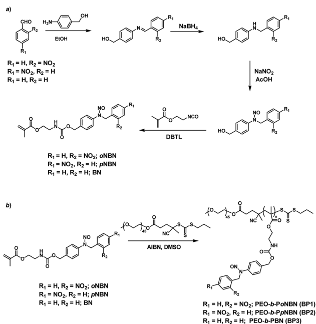
Scheme 2 Synthetic routes of (a) NO-releasing monomers, o NBN, p NBN, and BN and (b) amphiphilic diblock copolymers (BP1–BP3) through RAFT polymerization.
