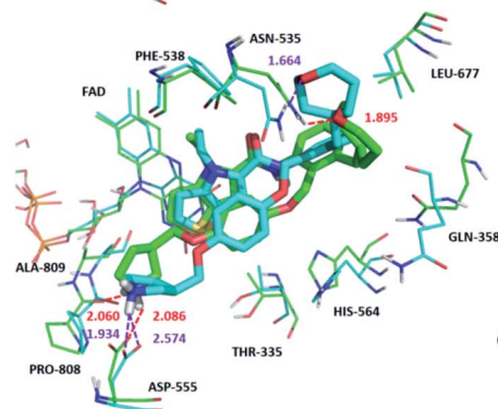
Fig. 12 The superposition of the docking structures and MD average structures of compound D4 (A), D5 (B), D8 (C). Carbon atoms of docking result and MD average structure are shown in green and cyan, respectively. H-bond of docking result and 50 ns MD result are shown in red dash line and purple dash line, respectively.
