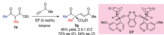
Scheme 11 Asymmetric 1,4-addition of \beta -ketoester to alkynone using catalyst C7 .
