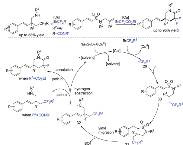
Scheme 15 The difunctionalization of unactivated alkenes through desulfonation.
