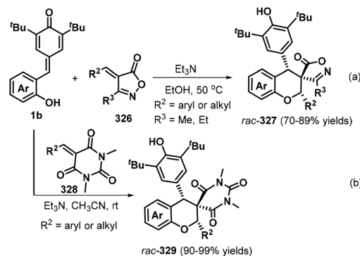
Scheme 73 Synthesis of spirochromans.
