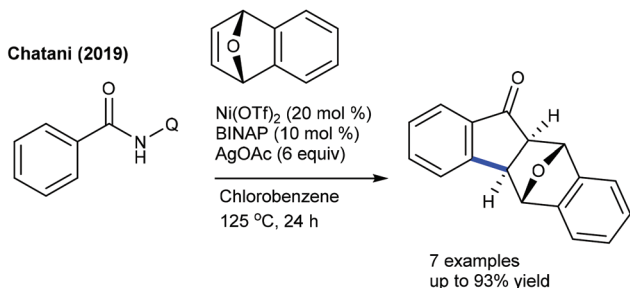
Scheme 130 Reaction of benzamides with oxabenzonorbornadienes.
