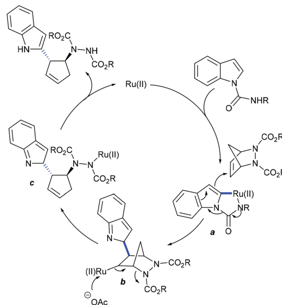
Scheme 74 Mechanism of C2-functionalization of indoles with heterobicyclic alkenes.
