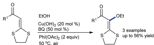
Scheme 148 Ethoxylation of cyclic \alpha -aryloxyketene dithioacetal.
