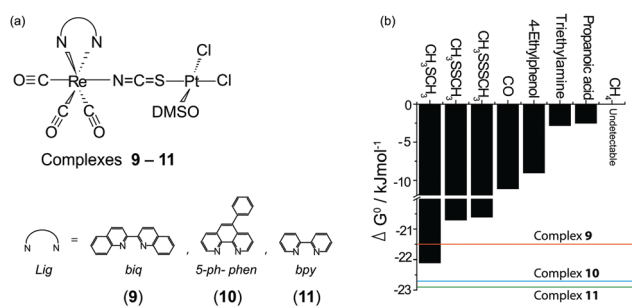
Fig. 6 (a) Structures of complexes 9–11 ; (b) binding strengths ( \Delta G^\circ ) of the [\text{Pt}^{II}(\text{DMSO})\text{Cl}_2\text{-analyte}] adducts. The three horizontal lines represent the \Delta G^\circ values of complexes 9–11 .
