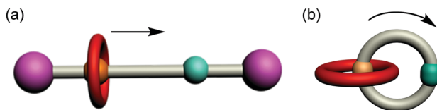
Fig. 1 Cartoon illustrations of mechanical motions: (a) translocation in typical [2]rotaxanes; (b) circumrotation in typical [2]catenanes.
