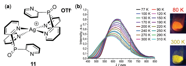
Fig. 10 (a) Molecular structure of Ag(I) complex 11 . (b) Normalized temperature-dependent emission spectral changes in the range of 77 – 310 \text{ K} . The pictures on the right show the solid emission colors of the samples at 80 and 300 \text{ K} , respectively. Reprinted with permission from ref. 77. Copyright 2019 the Partner Organisations.
