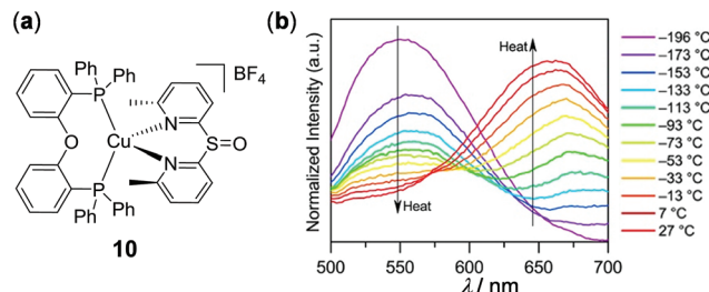
Fig. 9 (a) Molecular structure of Cu(I) complex 10 . (b) Normalized temperature-dependent emission spectral changes of 10 from -196 to 27^\circ\text{C} as thin films by drop-casting on quartz from MeOH solution ( \lambda_{\text{ex}} = 380 \text{ nm} ). Reprinted with permission from ref. 99. Copyright 2018 American Chemical Society.
