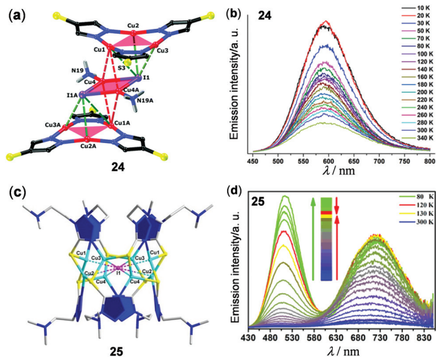
Fig. 21 (a) Crystal structure of the \text{Cu}_3\text{--Cu}_2\text{--Cu}_3 cluster 24 . (b) Temperature-dependent solid-state luminescence spectra of 24 monitored from 10 K to 340 K ( \lambda_{\text{ex}} = 345 \text{ nm} ). Reprinted with permission from ref. 118. Copyright 2018 The Royal Society of Chemistry. (c) Perspective view of the [\text{I}@\text{Cu}_8] cluster 25 viewed along the a axis. (d) Normalized temperature-dependent emission spectra of 25 in the solid state within the temperature range of 80–300 K. Reprinted with permission from ref. 119. Copyright 2017 American Chemical Society.
